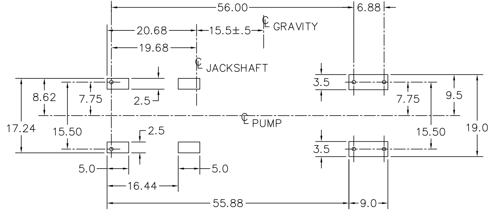
MOUNTING HOLES WITHOUT SKID
